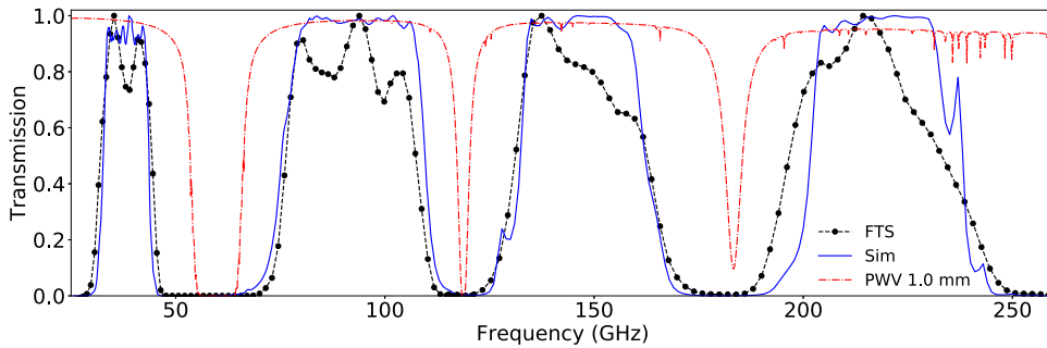
Figure 1. Average measured (dotted black) and simulated (solid blue) spectral response for different CLASS frequency bands overlapped with the atmospheric transmission model at the CLASS site with PWV = 1 mm (red dashed-dotted). The atmospheric transmission model was obtained from the Atacama Large Millimeter/submillimeter Array (ALMA) atmospheric transmission calculator based on the ATM code described in Pardo et al. (2001). The spectral response is normalized to unit peak, and the atmospheric transmission model is in units of fractional power transmitted. The bandwidths and center frequencies for different diffuse sources for these passbands are shown in Table 2.
